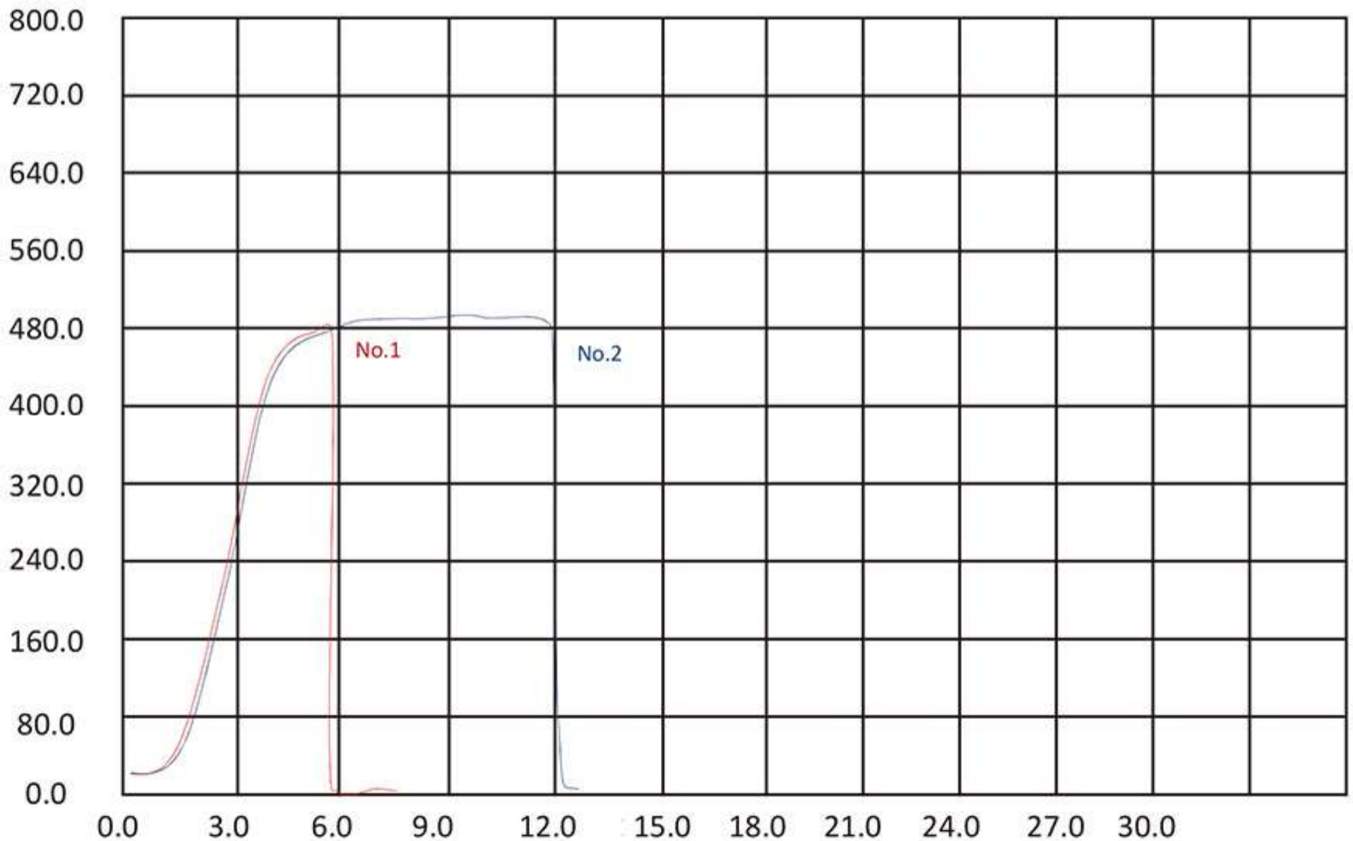
[Load 0.0 / 800.0 kgf Load] versus [Time Pass 0.0 / 30.0 sec] 금속 : 평판인장시험
